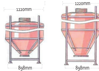
90° CONE 200mm OUTLET
